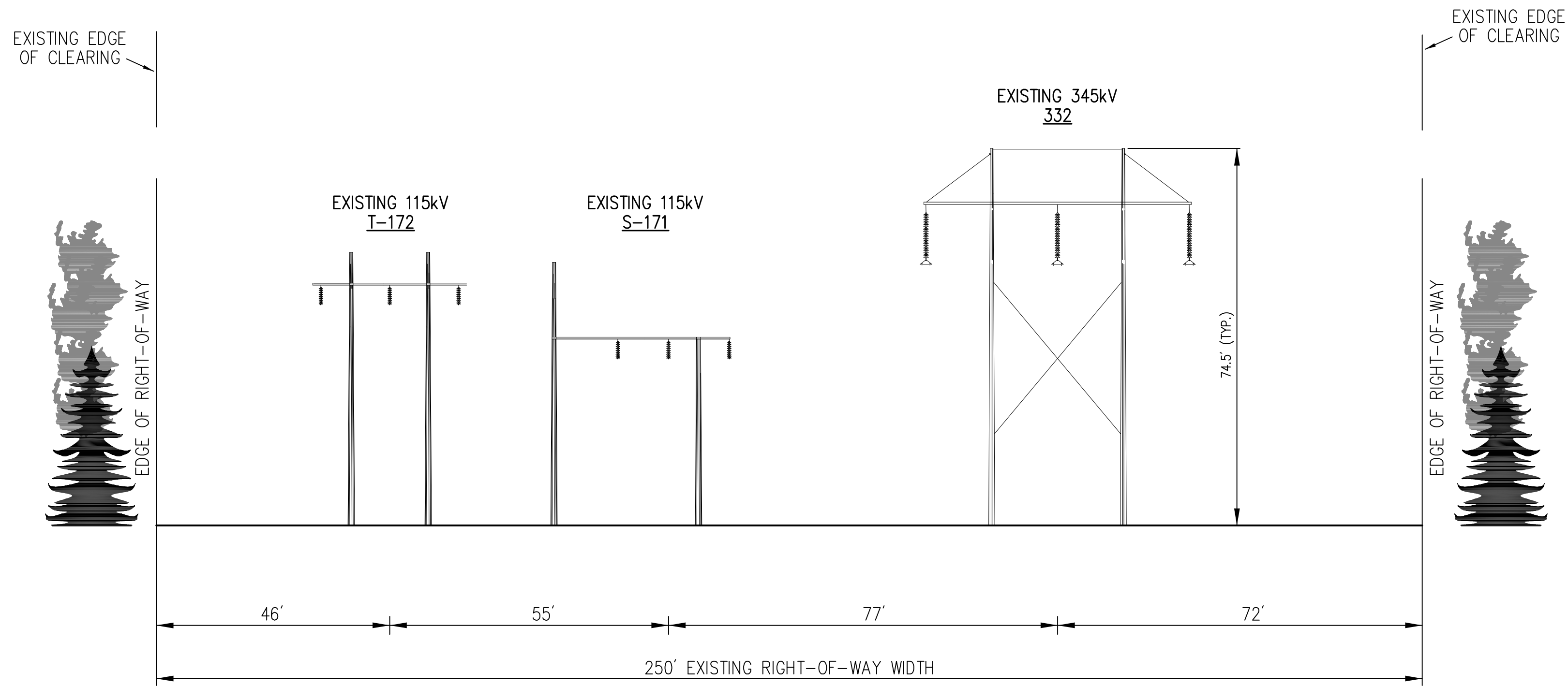
Existing Cross Section
