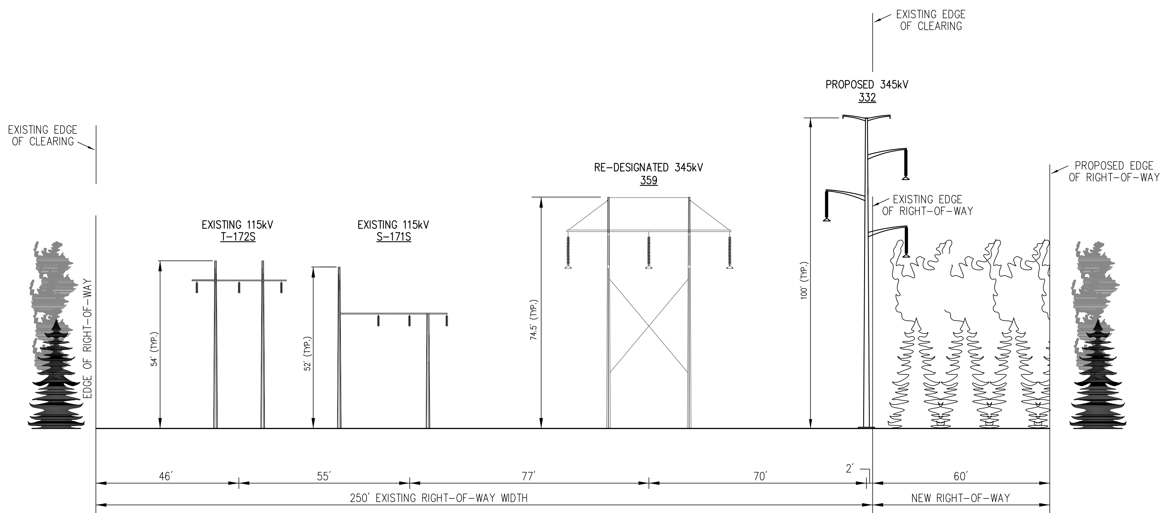
West Warwick Alternative Cross Section
