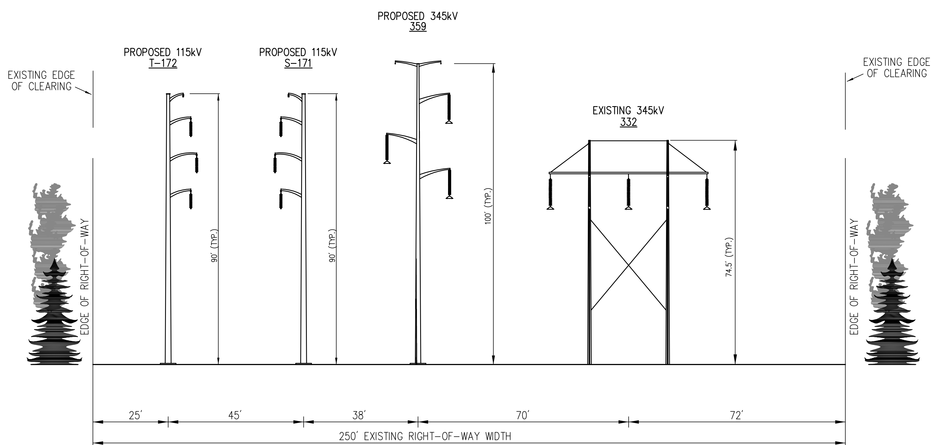
Proposed Cross Section
